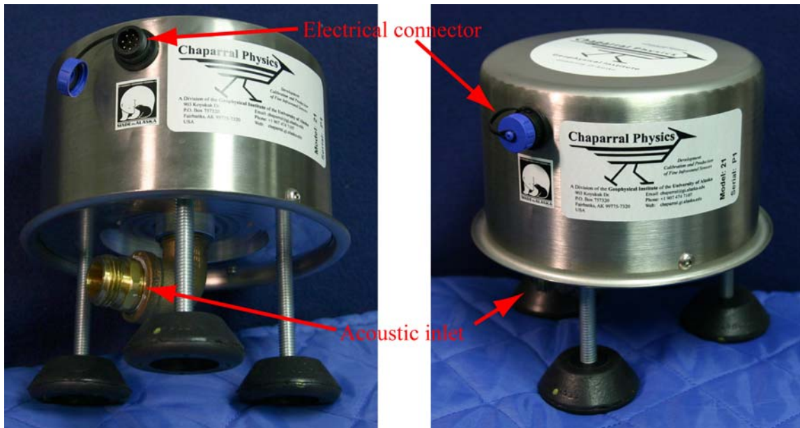
A Chaparral Physics Model 21 infrasond sensor.
